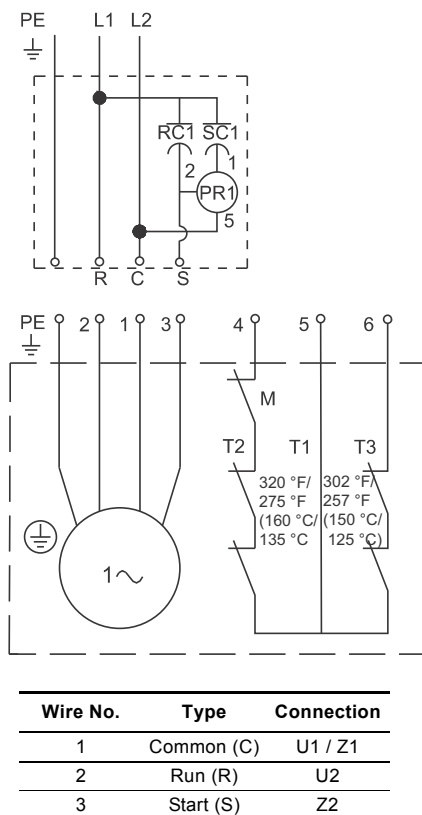
Fig. 12 Wiring diagram for single-phase SEG pumps. See table below.
