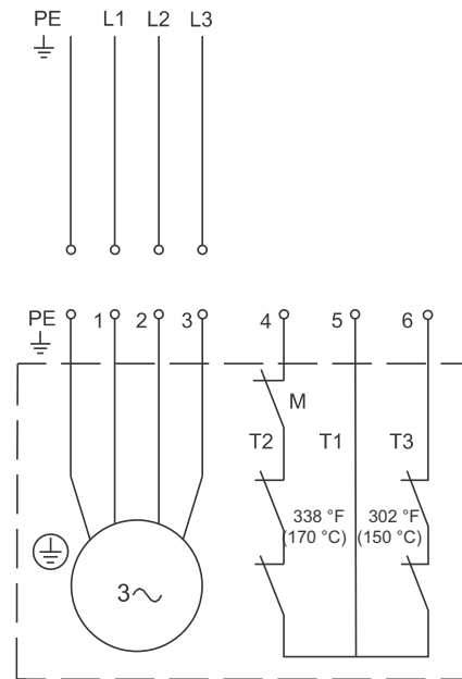
Fig. 13 Wiring diagram for three-phase SEG pumps
