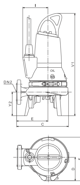
Fig. 16 Free-standing installation with foot extensions
