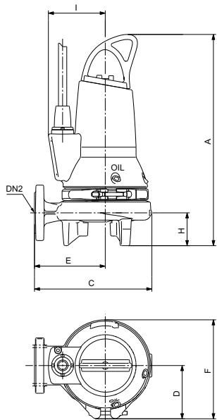
Fig. 15 Free-standing installation
